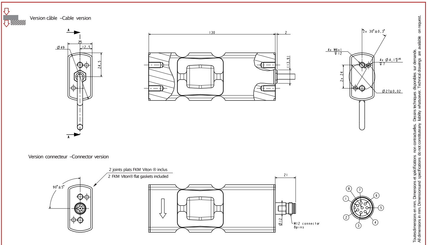
Câblage version câble –Wiring cable version
